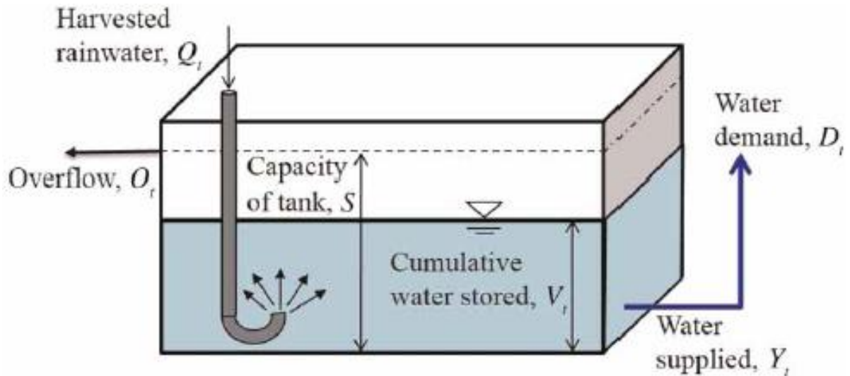
Figure 3-1: Schematic diagram of rainwater fluctuation in the tank
