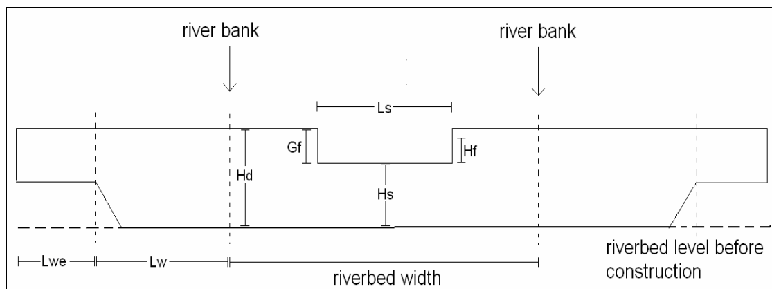
Figure 3-2: Cross-sectional width dimensions for a typical sand dam construction
